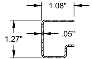
STILE REINFORCEMENT STEEL
